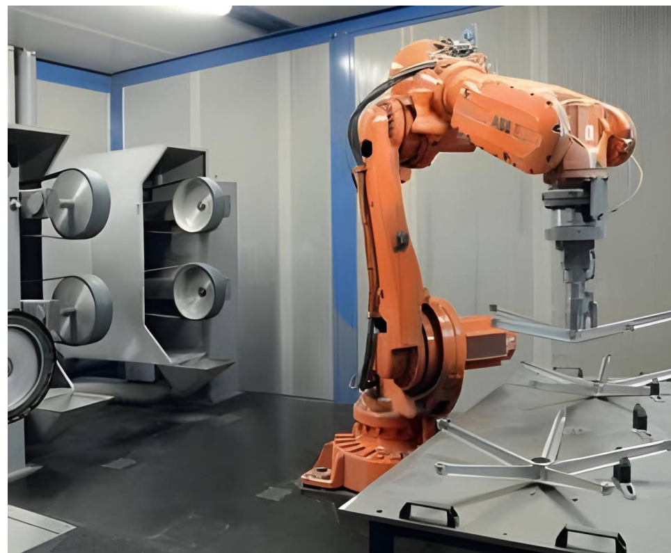
Robotic Precision Polishing
